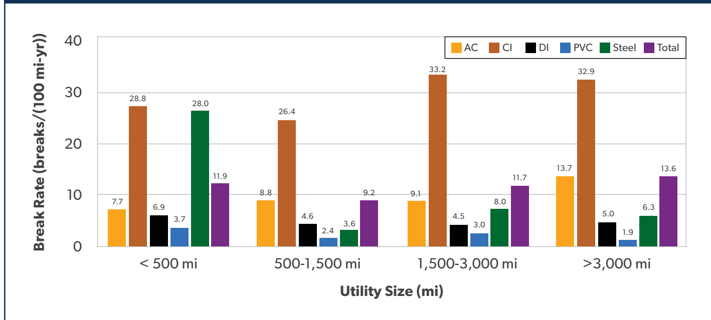
FIGURE 34: BREAK RATES BY UTILITY SIZE FOR 5-YEAR PERIOD (BASIC SURVEY)
