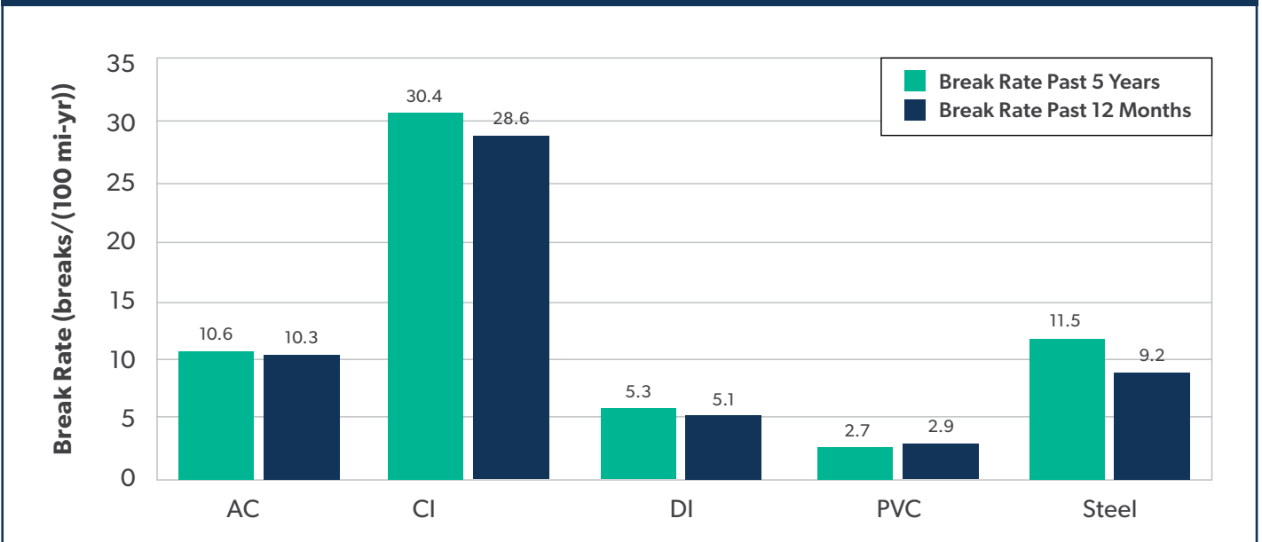
FIGURE 29: BREAK RATES BY PIPE MATERIAL FOR A 12-MONTH AND 5-YEAR PERIOD (BASIC SURVEY)
