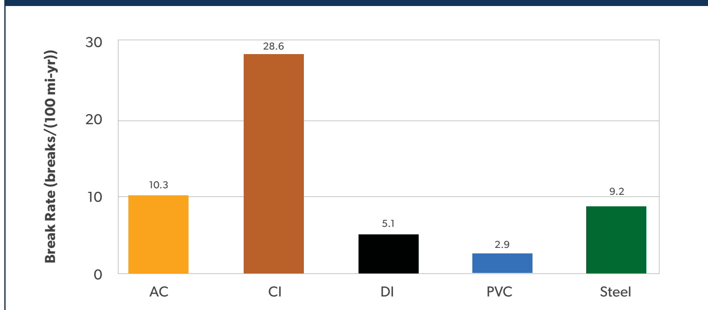
FIGURE 52: OVERALL BREAK RATES OF PIPE MATERIAL (BASIC SURVEY)
