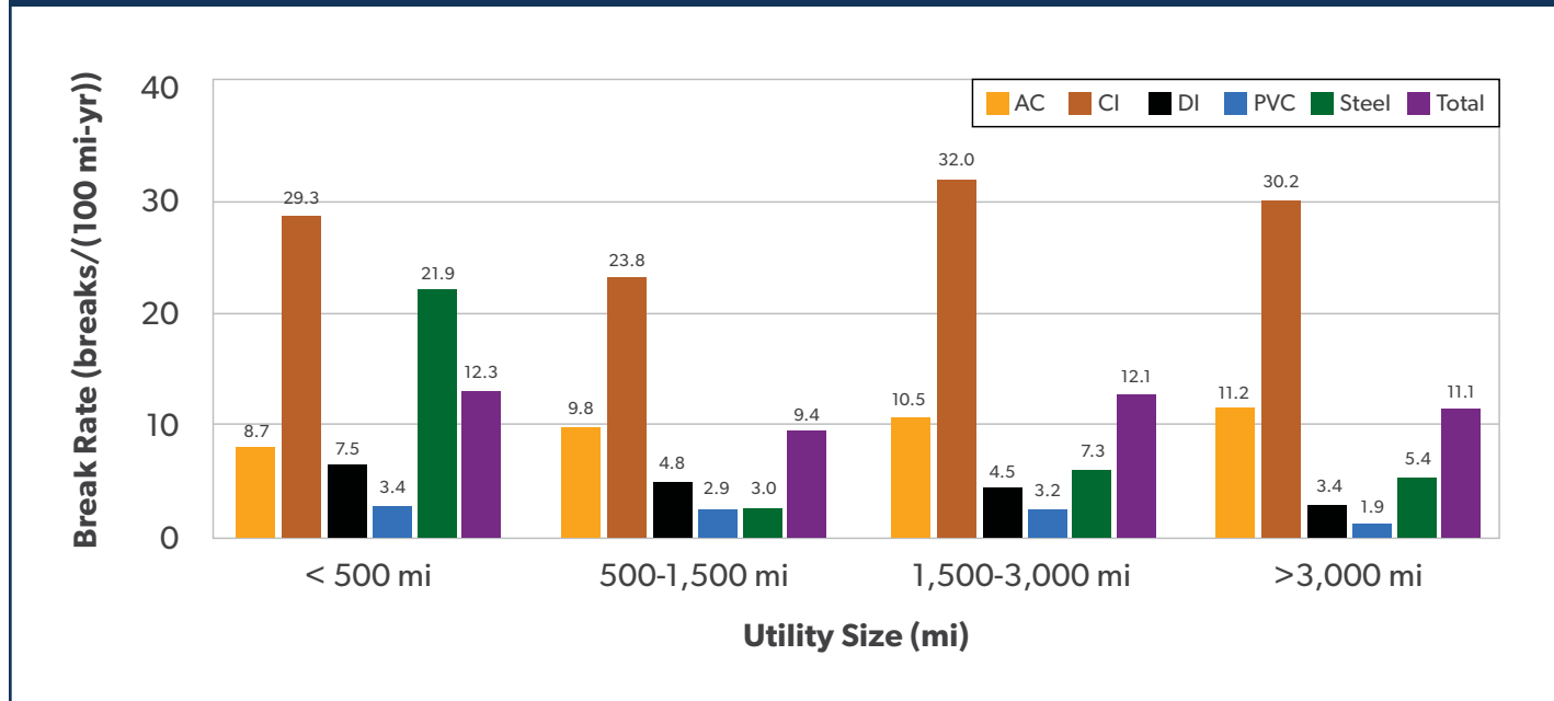
FIGURE 33: BREAK RATES BY UTILITY SIZE FOR 12-MONTH PERIOD (BASIC SURVEY)
